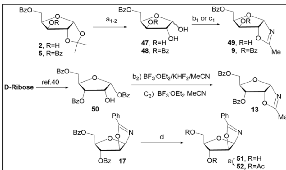
Scheme 6. Synthesis of acylated D-xylo-, ribo- and arabinofuranosyl oxazolines. Reagents and conditions: ( a_1 ) 2 , 93% aq TFA, rt, 2 h, 47 , 80%; ( a_2 ) 5 , 93% aq TFA, rt, 2 h, 48 , 80%; ( b_1 ) benzoylated D-xylofuranoses 47-48 , \text{CH}_3\text{CN} , \text{KHF}_2\cdot\text{BF}_3\cdot\text{Et}_2\text{O} , rt, 3-4 h, 5 % aq \text{NaHCO}_3 , 49 , 75%; 9 , 99%; ( c_1 ) 48 , \text{CH}_3\text{CN}/\text{BF}_3\cdot\text{Et}_2\text{O} , rt, 3 h, 5 % aq \text{NaHCO}_3 , 9 , 65%; ( b_2 ) 50 , \text{CH}_3\text{CN} , \text{KHF}_2\cdot\text{BF}_3\cdot\text{Et}_2\text{O} , rt, 3 h, 1N aq \text{NaOH} , 13 , 99%; ( c_2 ) 50 , \text{CH}_3\text{CN} , \text{BF}_3\cdot\text{Et}_2\text{O} , rt, 3 h, 1N aq \text{NaOH} , 13 , 65%; d) 17 , \text{NH}_3/\text{MeOH} , rt, 18 h, 51 , 93%; e) 51 , \text{Ac}_2\text{O} , Py, rt, 52 , 80%.
