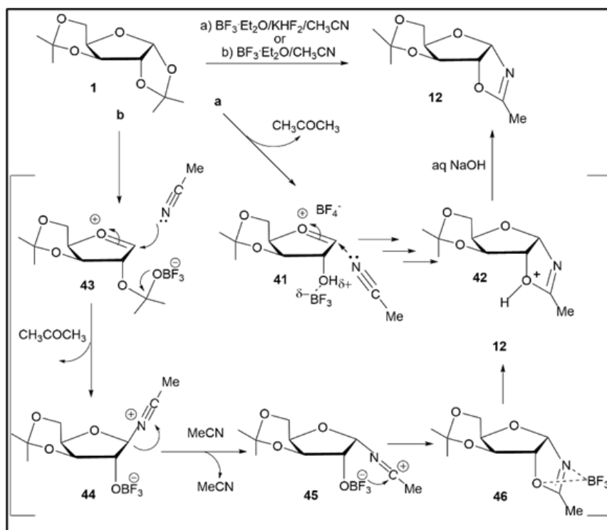
Scheme 5. Proposed intermediates during \text{BF}_3\cdot\text{Et}_2\text{O} -promoted reactions of diacetone 1 with acetonitrile
