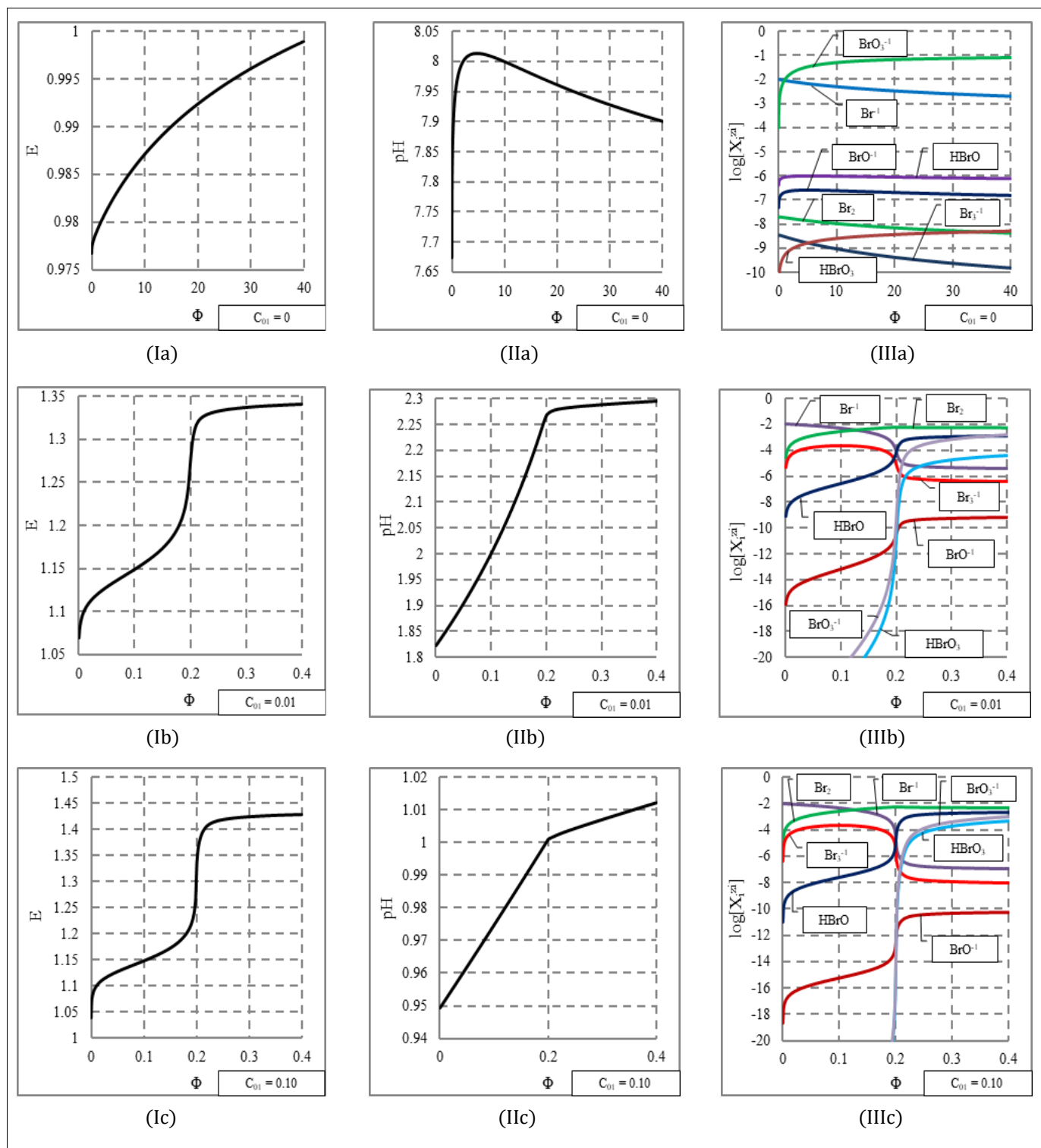
Fig. 1: The functions: E = E(\Phi) (column I), pH = pH(\Phi) (column II) and speciation diagrams (column III), at (C_0, V_0, C) = (0.01, 100, 0.1) , and three different C_{01} values, indicated at the graphs.
